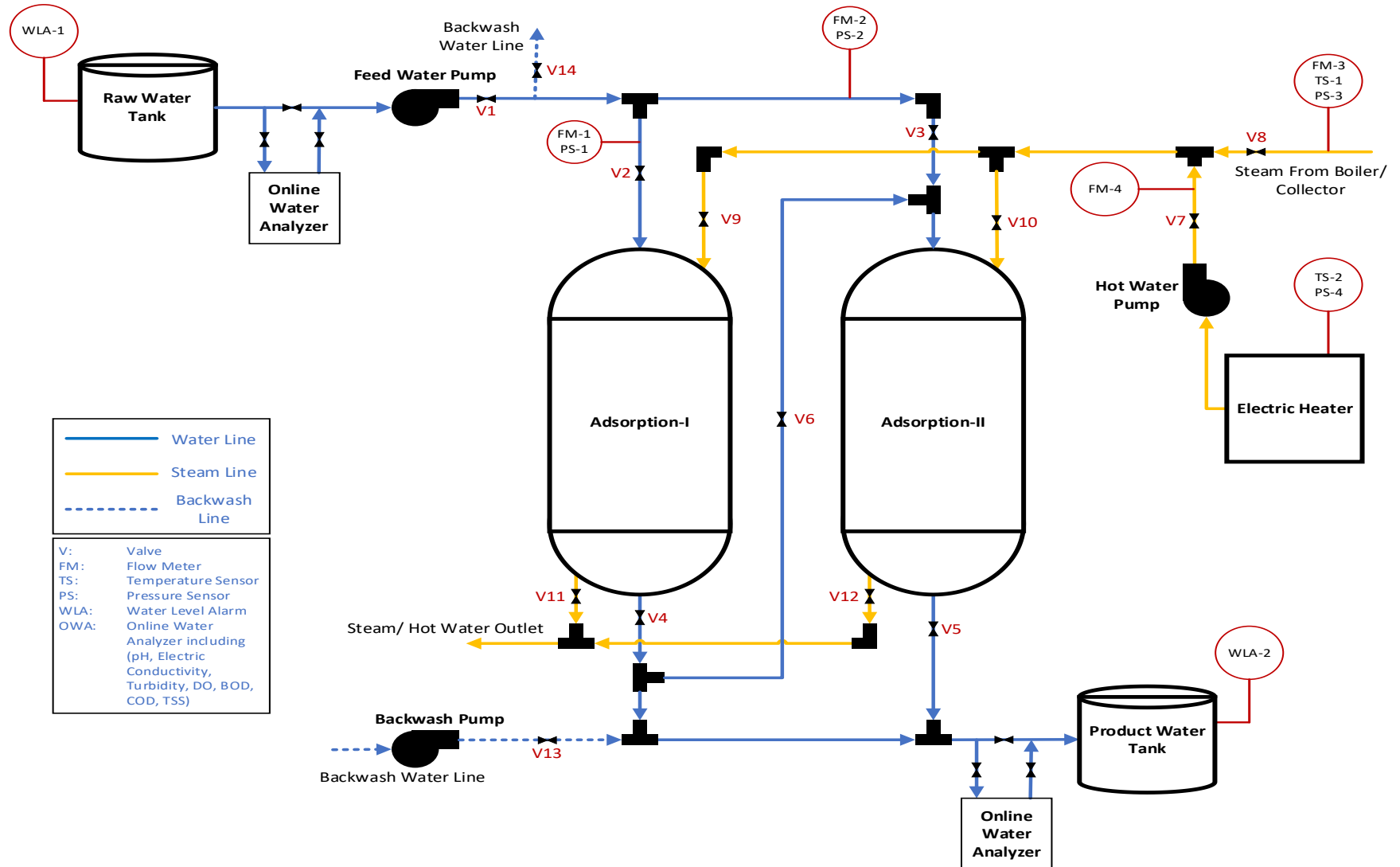
Fig 2: P&ID Diagram of Adsorption system
