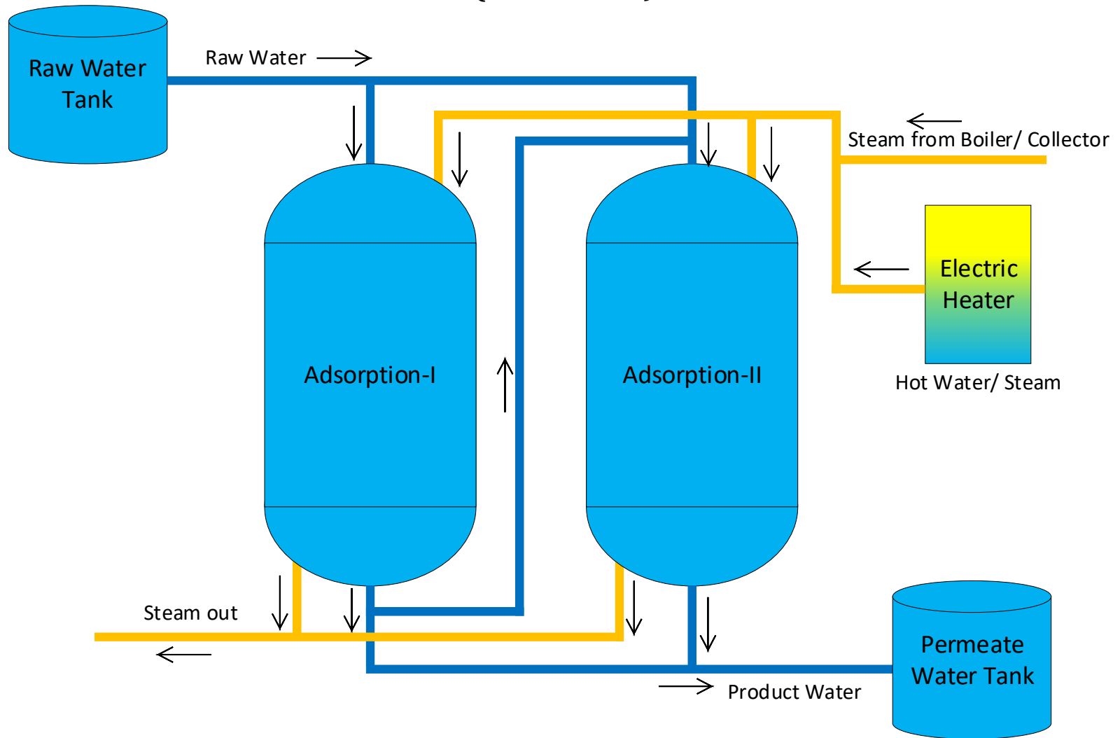
Fig 1: Schematic Diagram of Adsorption system
