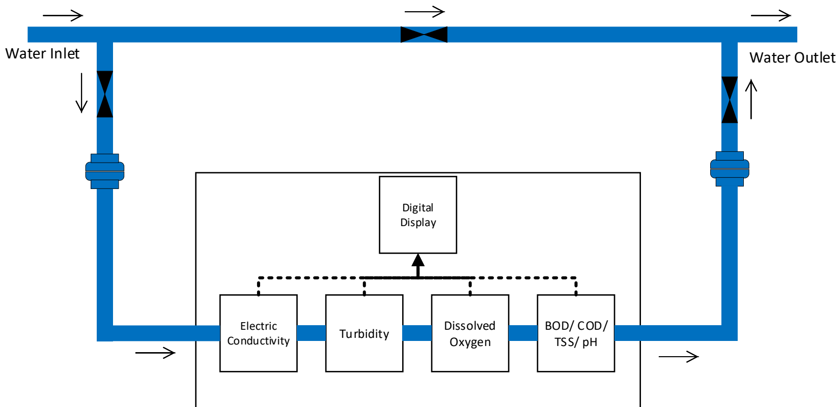
Fig 3: Online Water Test Analyzer Test Rig
